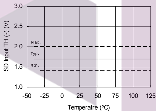
Figure 22A. SD Input TH(-) vs. Temperature
