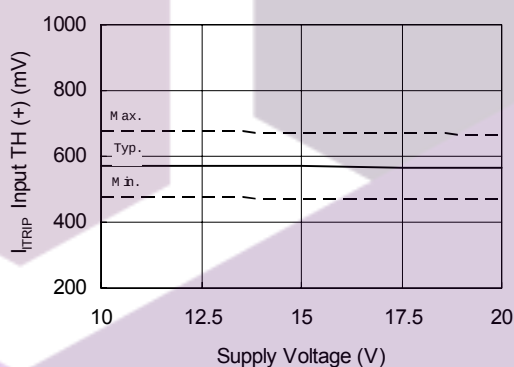
Figure 23B. I_{TRIP} Input TH(+) vs. Voltage
